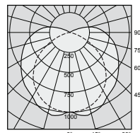
FL98016 - Viking LED Batten 4K Mains ULOR: 10% DLOR: 90%
